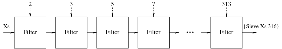
Figure 4.12: Pipeline of filters generated by {Sieve Xs 316} .
