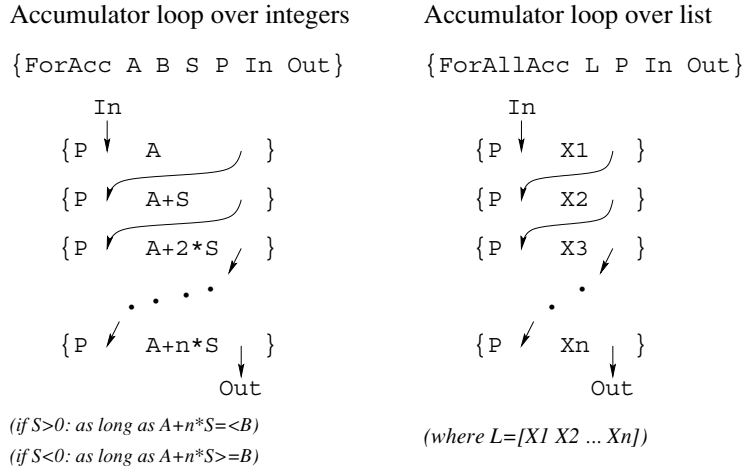
Figure 3.26: Accumulator loops over integers and lists.
