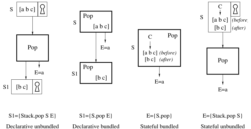
Figure 6.3: Four versions of a secure stack.
