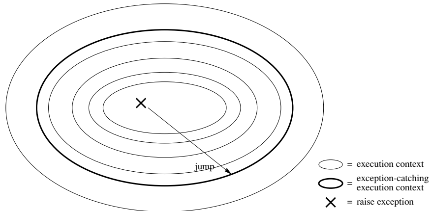
Figure 2.21: Exception handling.
