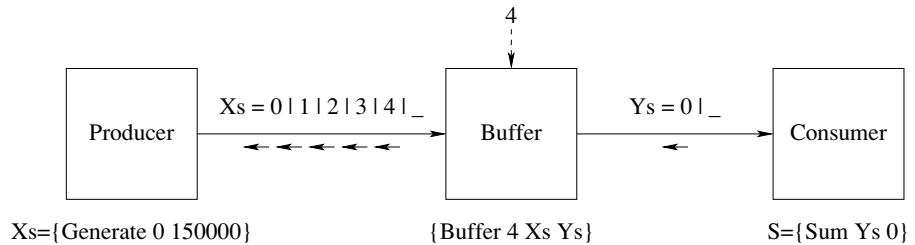
Figure 4.13: Bounded buffer.
